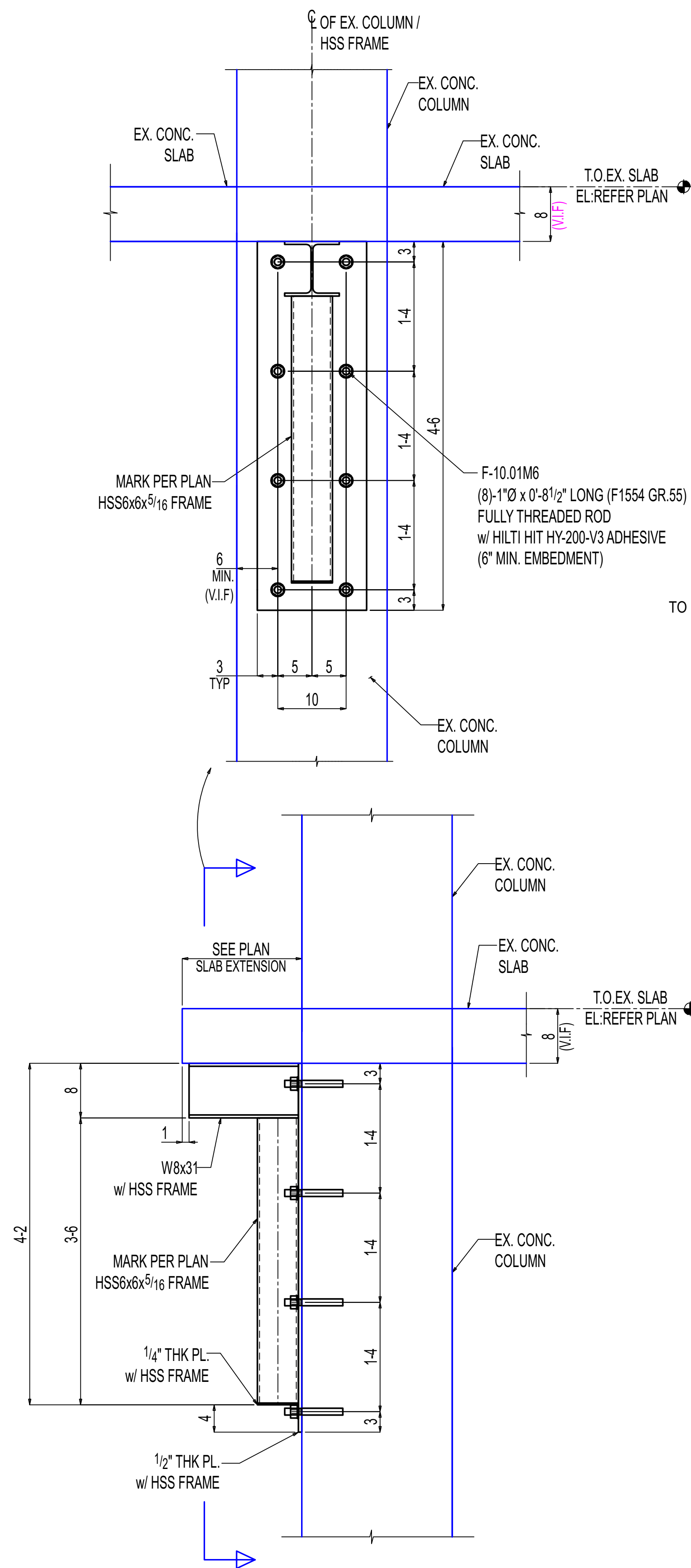
A-A (NEW SLAB EXTENSION SUPPORT 1'-6" TO 3'-1") E-10.00 (REF:11/S314) OTHERS NOT SHOWN FOR CLARITY
