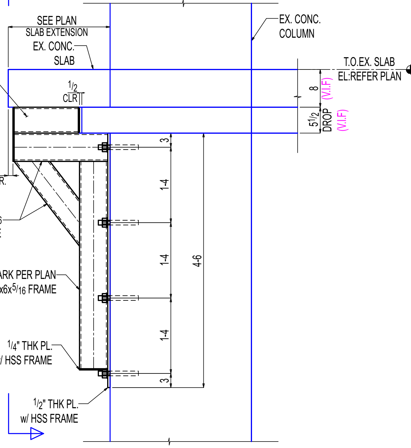
B-B E-10.00 (REF: 3 & 4/S307) OTHERS NOT SHOWN FOR CLARITY
